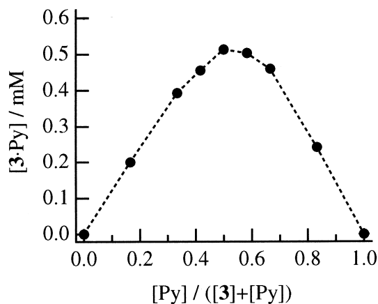
Figure 3. Job's plot of [3-Py] estimated from chemical shift change of the ortho -proton in pyridine ([3]+[Py]=1.2 mM, in benzene- d_6 , at 25 °C).
