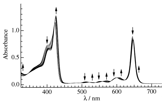
Figure 1. Absorption spectral change in dry benzene solution of zinc chlorin 3 ( =12\mu\text{M} ) by addition of pyridine ( =0\text{--}340\mu\text{M} ) at 25^\circ\text{C} . Arrows show the direction of absorbance change with addition of pyridine.
