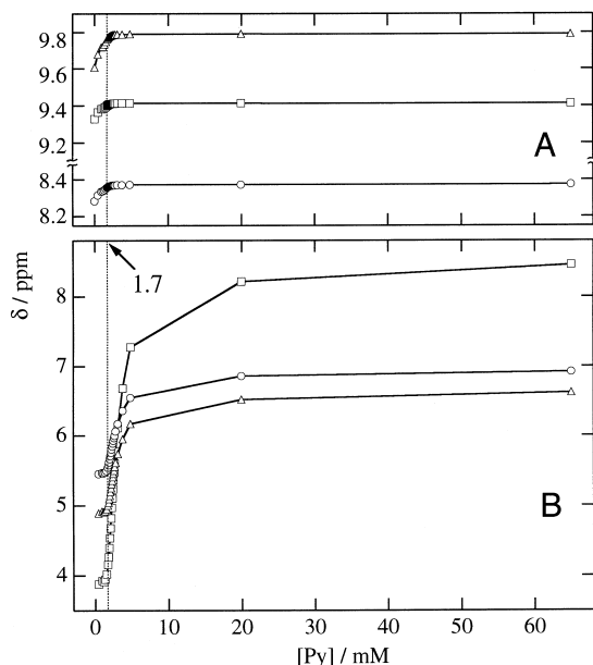
Figure 2. Change of chemical shifts ( \delta ) of (A) 5-H ( \square ), 10-H ( \triangle ) and 20-H ( \circ ) of zinc chlorin 3 (=1.7 mM) and (B) o-H ( \square ), m-H ( \triangle ), and p-H ( \circ ) of additive pyridine (=0–65 mM) in benzene- d_6 at 25 °C.
