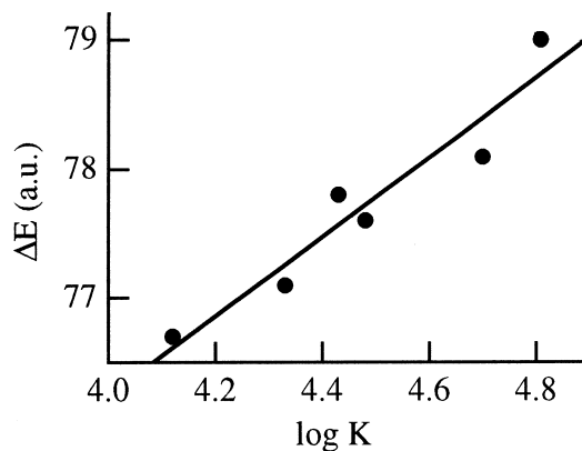
Figure 4. Dependency of \Delta E calculated from molecular modeling with \log K observed from visible spectral change.
