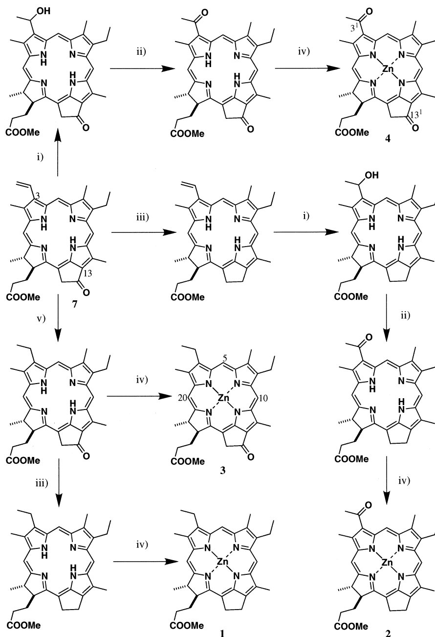
Scheme 1. i) HBr–AcOH (55°C), \text{CH}_2\text{N}_2/\text{Et}_2\text{O} ; ii) \text{Pr}_4\text{NRuO}_4\text{–Me}(\text{O})\text{N}(\text{CH}_2\text{CH}_2)_2\text{O}/\text{CH}_2\text{Cl}_2 ; iii) \text{NaBH}_4\text{–TFA}/\text{CH}_2\text{Cl}_2 (0°C); iv) \text{Zn}(\text{OAc})_2\cdot 2\text{H}_2\text{O}/\text{MeOH–CH}_2\text{Cl}_2 ; v) \text{H}_2/\text{Pd–C}/\text{CH}_3\text{COCH}_3 .
